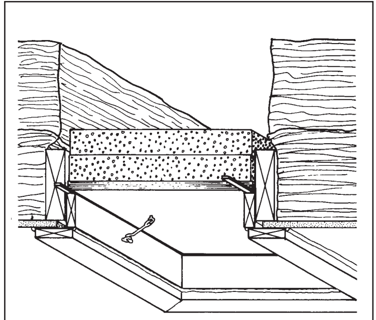
Cutaway view of a well-sealed attic hatch
