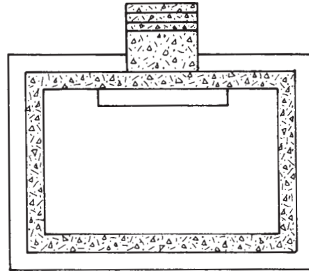
Overlap interior and exterior insulation
