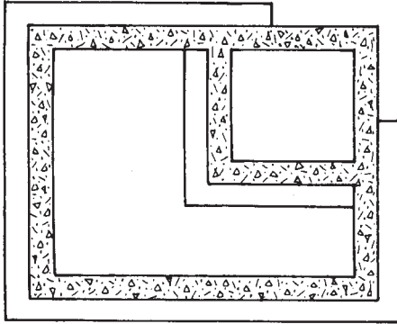
Insulating a cold room on the interior
