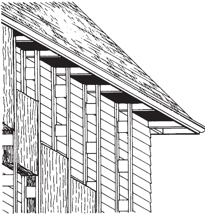
Trusses can be hung from the rafters and nailed to the existing wall.
